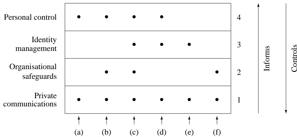
Figure 3: Layered version of the privacy architecture
