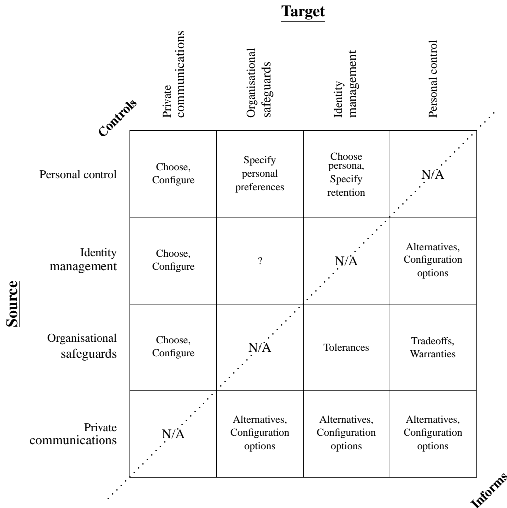
Figure 2: Examples of how the upper layers of the architecture control the lower layers and how the lower layers inform the upper layers
