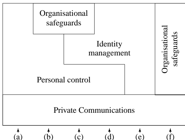
Figure 1: Working version of the privacy architecture
